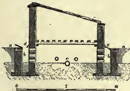
FIG. 10.—Ventilated Plant Pit.
